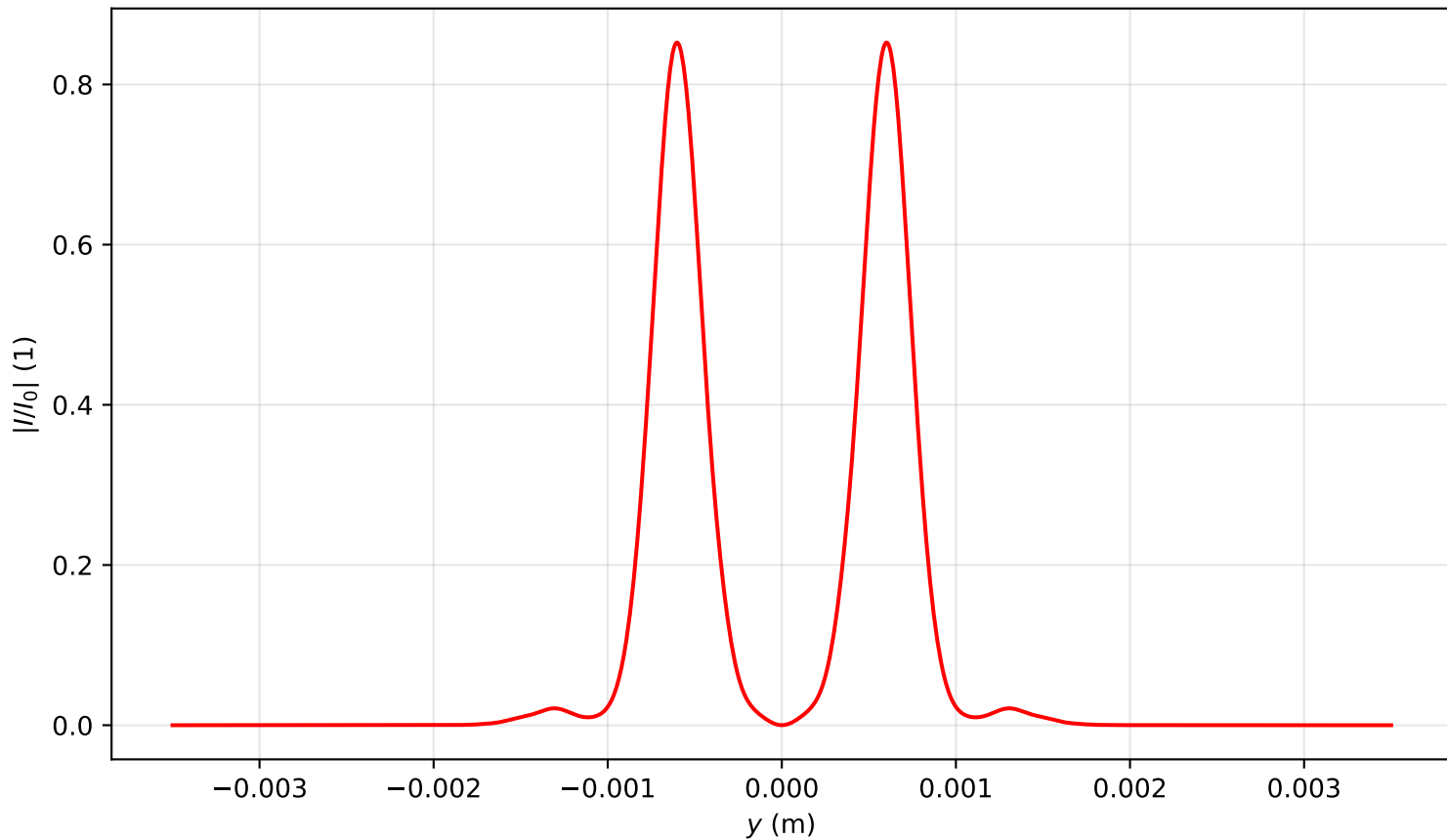
Intensity profile I(x=0, y, z=1.035)/I_0 , P_{in}=6.0P_{cr} , artificial time
